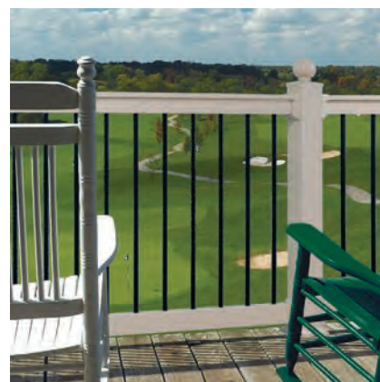
"B" Series Baluster 3/4" Round Aluminum 3-7/8" Baluster Spacing See Page 1 for Baluster Colors
