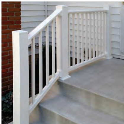
Standard Baluster 7/8" x 1-1/2" Rectangular Vinyl 2-7/8" Baluster Spacing
